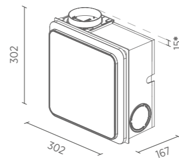
FLAT- e IN 300 Ø 100 - 120 mm Sporgenza 38 mm / protrusion
