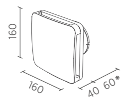
ALBA 10/4" Ø 100 mm
