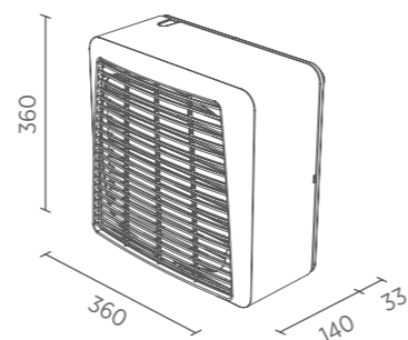
EASY 30/12" Ø 324 - 337 mm
